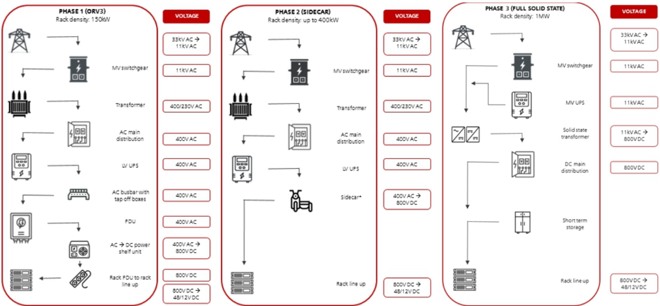
Figure 11: Three phases of 800V DC architecture
