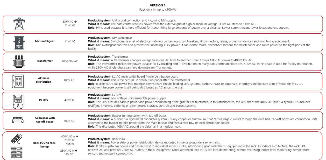
Figure 12: Current data centre architecture (version 1)
